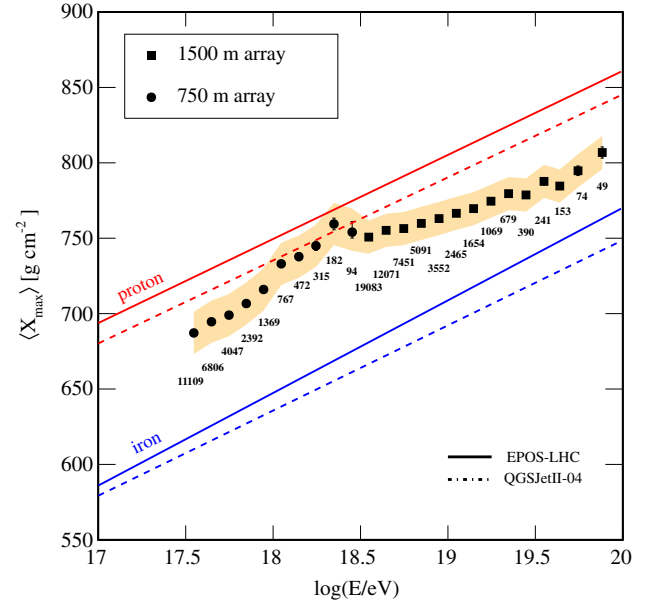
FIG. 15. Mean values of the X_{\max} distributions obtained with the data of the 750 and 1500 m surface arrays as a function of the energy. The shaded area indicates the systematic uncertainties. Data are compared to the predictions from simulations of protons and iron nuclei for two different hadronic models. The number of selected events in each energy bin is indicated.
