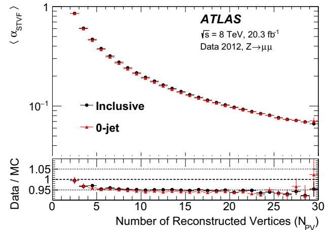
Fig. 2 The mean \alpha_{STVF} weight is shown versus the number of reconstructed vertices ( N_{PV} ) for 0-jet and inclusive events in Z \rightarrow \mu\mu data. The inset at the bottom of the figure shows the ratio of the data to the MC predictions with only the statistical uncertainties on the data and MC simulation. The bin boundary always includes the lower edge and not the upper edge
