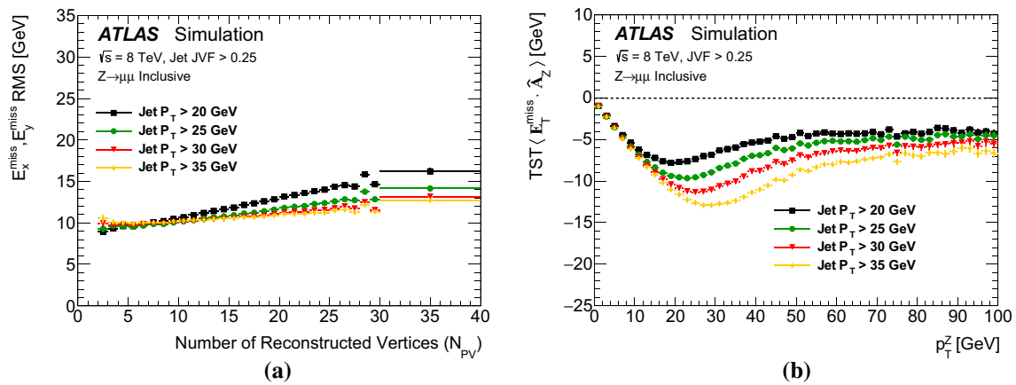
Fig. 19 The a TST E_T^{\text{miss}} resolution as a function of the number of reconstructed vertices per bunch crossing ( N_{PV} ) and the b TST \vec{E}_T^{\text{miss}} in the direction of the \vec{p}_T^Z are shown for different jet- p_T thresholds using
