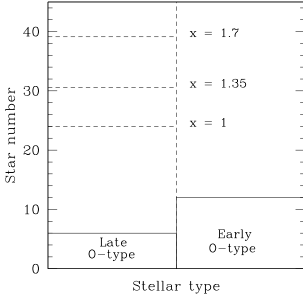
Fig. 1. Expected numbers of late-type stars (left column, horizontal dashed lines) given the number of early-type stars (right column) in the catalogue of PACWBs for different assumptions on the IMF index x . The solid horizontal lines stand for the numbers found in the current catalogue of PACWBs.
