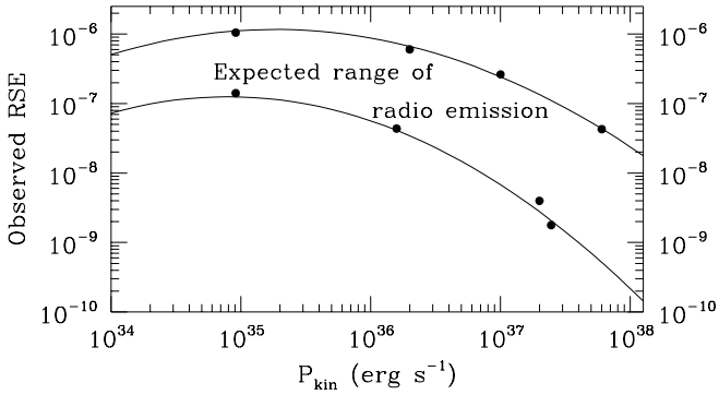
Fig. 2. Rough estimate of the expected region of radio emission as a function of the kinetic power based on the radio synchrotron efficiency (RSE) derived for the members of the catalogue of PACWBs (truncated banana diagram). The two curves correspond to Eqs. (1) and (2). The black bullets represent the data points used for the quadratic regression.
