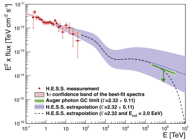
Figure 2. Photon flux as a function of energy from the Galactic center region. Measured data by H.E.S.S. are indicated, as well as the extrapolated photon flux at Earth in the EeV range, given the quoted spectral indices (Abramowski et al. 2016; conservatively the extrapolation does not take into account the increase of the p - p cross-section toward higher energies). The Auger limit is indicated by a green line. A variation of the assumed spectral index by \pm 0.11 according to systematics of the H.E.S.S. measurement is denoted by the light green and blue band. A spectral index with cutoff energy E_{\text{cut}} = 2.0 \cdot 10^6 \text{ TeV} is indicated as well.
