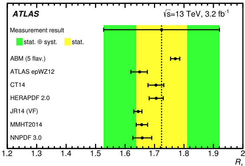
Figure 6. Comparison between observed and predicted values of R_t = \frac{\sigma_t}{\sigma_{\bar{t}}} . Predictions are calculated at NLO precision [7, 8] in the five-flavour scheme and given for different NLO PDF sets. The uncertainty includes the uncertainty in the renormalisation and factorisation scales, as well as the combined internal PDF and \alpha_s uncertainty. The dotted black line indicates the measured value. The combined statistical and systematic uncertainty of the measurement is shown in green, while the statistical uncertainty is represented by the yellow error band. Predictions for all presented PDF sets are within the statistical uncertainty of the measurement.
