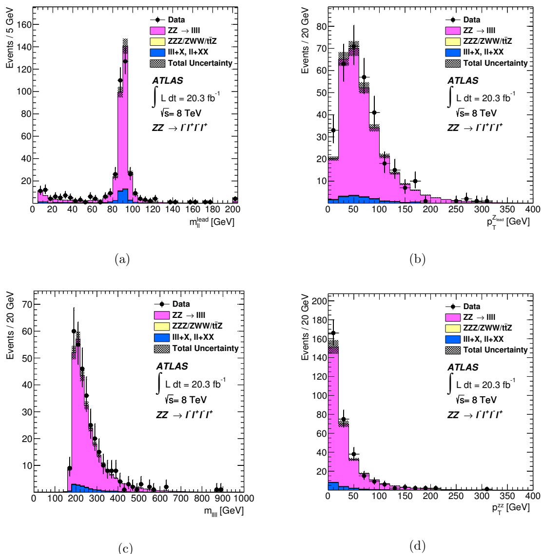
Figure 2. Kinematic distributions for ZZ \rightarrow \ell^- \ell^+ \ell'^- \ell'^+ candidates in all four-lepton final states: (a) m_{\ell^- \ell^+}^{\text{lead}} , (b) p_T^{Z\text{lead}} , (c) m_{\ell^- \ell^+ \ell'^- \ell'^+} and (d) p_T^{ZZ} . The points represent the observed data and the histograms show the expected number of ZZ signal events and the background estimate. The shaded band shows the combined statistical and systematic uncertainties in the prediction and the background. No selection on the leading lepton pair mass is required for (a), while the full selection is applied for the other distributions.
