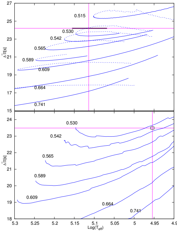
Figure 1. Average of the computed \ell = 1 period spacings for VV 47 (upper panel) and J0349 (lower panel) corresponding to our PG 1159 evolutionary sequences in terms of \log(T_{\text{eff}}) . Dashed (solid) lines correspond to evolutionary stages before (after) the “evolutionary knee”. Also shown are the observed period spacings and the T_{\text{eff}} , along with their uncertainties.
