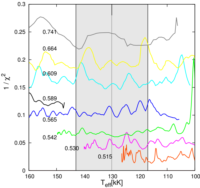
Figure 3. Same as Figure 2 but for VV 47, for the case “before the knee”. The curves have been arbitrarily shifted upward for clarity (with a step of 0.025).
