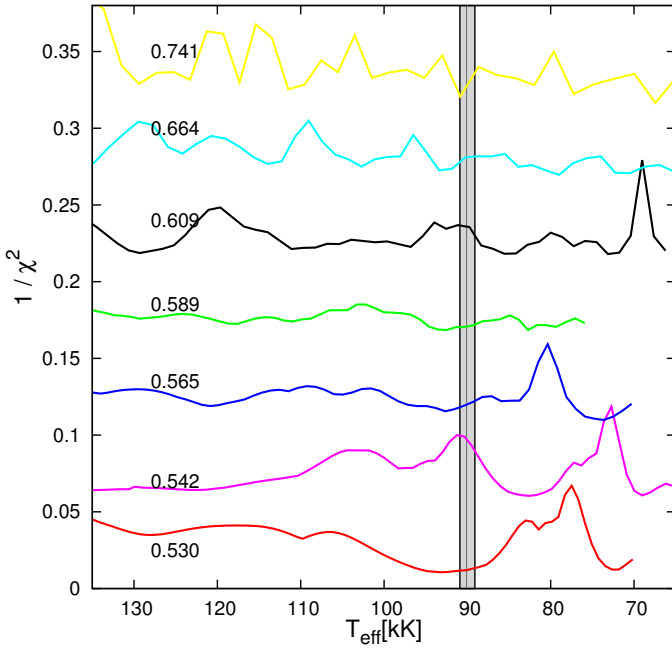
Figure 2. Inverse of the quality function of the period fit considering \ell = 1 g modes vs T_{\text{eff}} for J0349. The curves have been arbitrarily shifted upward for clarity (with a step of 0.05).
