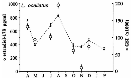
FIG. 2. Seasonal variations of gonadosomatic index (GSI) and plasma estradiol-17 \beta levels in female Leptodactylus chaquensis and Leptodactylus ocellatus . Each point is the mean of 10 determinations \pm SD.
