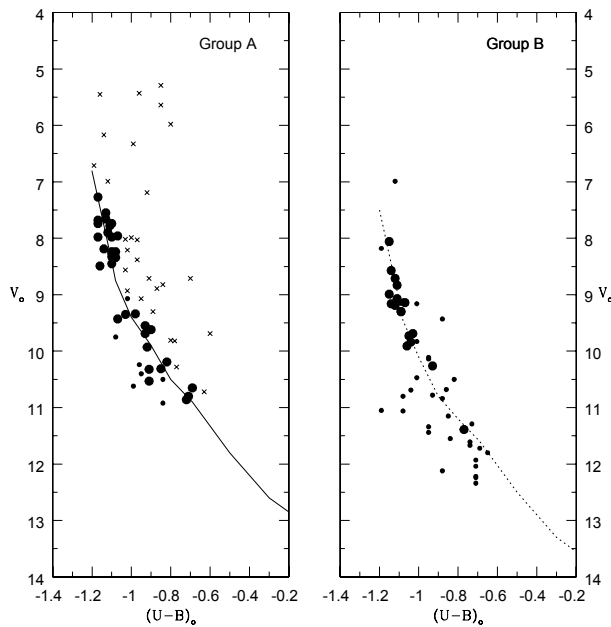
Fig. 1. V_0 vs. (U-B)_0 for members of Group A (Fig. 1a, left plot) and for young stars in Group B (Fig. 1b, right plot). Small points indicate magnitude and colors from photographic photometry, and crosses are used for non-members. The position of the ZAMS for Group A (full line) and a possible ZAMS for stars in Group B (dotted line), are also shown.
