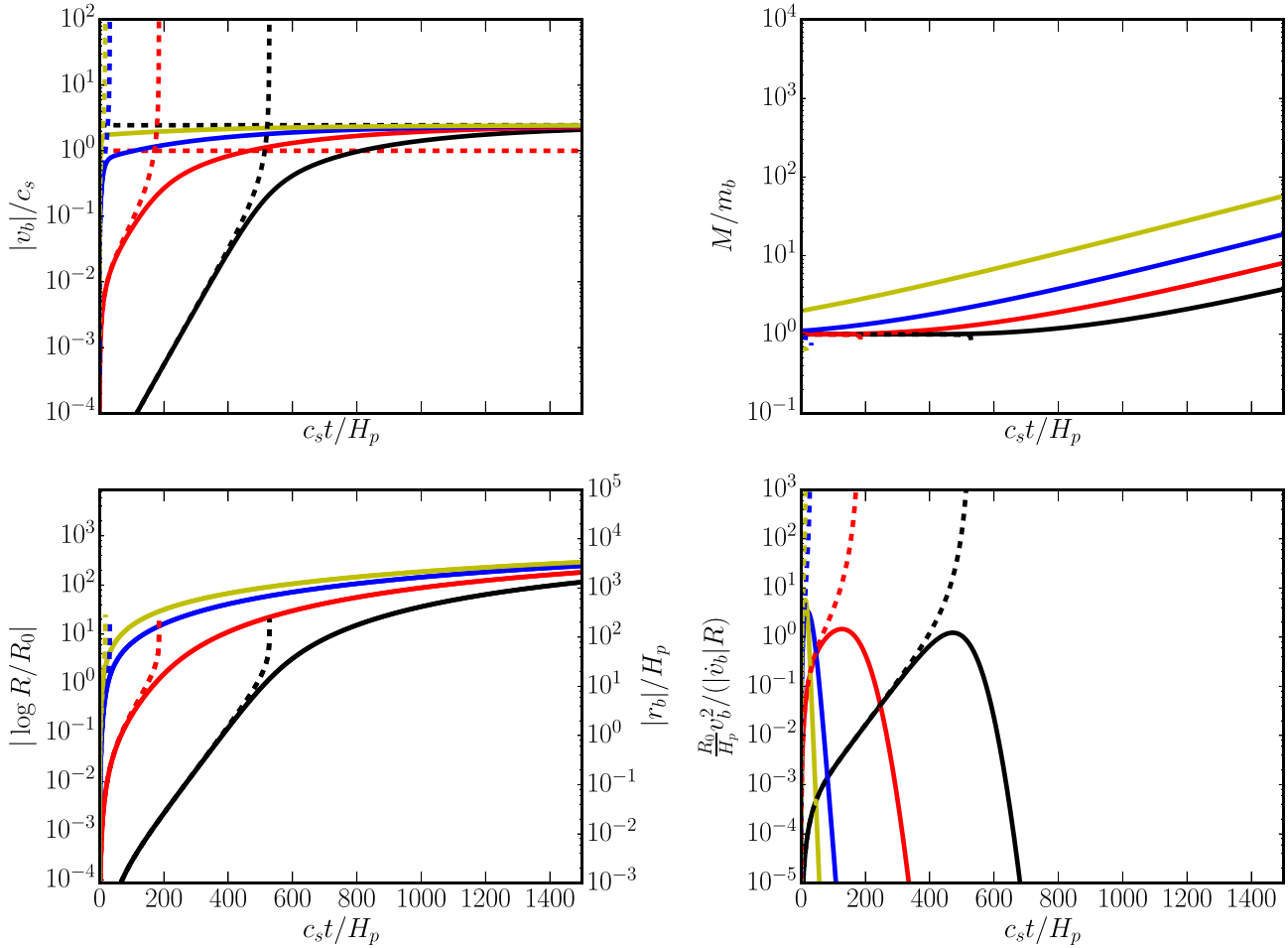
Figure 2. Same as Fig. 1 but for the case of \Delta\nabla = 10^{-3} .
