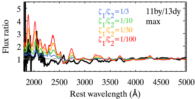
Figure 13. Same as the right-hand panel of Fig. 12, but using the flux-ratio spectrum of SN 2011by and SN 2013dy instead.
