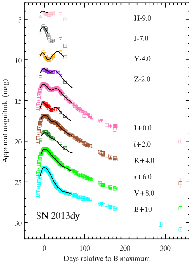
Figure 1. The KAIT BVRI and RATIR rZYJH light curves of SN 2013dy. The solid lines represent the best fit (from snopy ) to the observed light curves.
