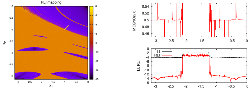
Fig. 8 (a) (left): The RLI mapping on gray-scale (color online) plot composed of 10^6 initial conditions, for 10^5 iterations (in logarithmic scale); (b) (right): The MEGNO(2,0), the LI and the RLI final values for 10^3 initial conditions along the line x_2 = -3 , for 10^5 iterations (the LI and the RLI final values are in logarithmic scale).
