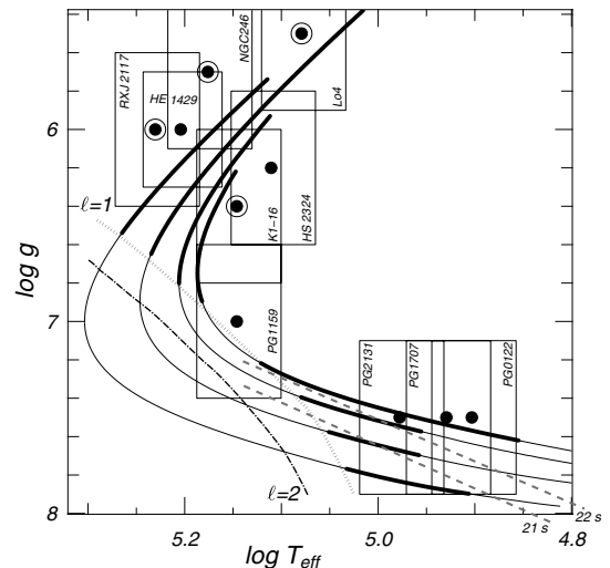
Fig. 4. The GW Vir instability domains on the \log T_{\text{eff}} - \log g plane. The dots represent observed variable PG 1159 stars. Encircled dots indicate the pulsators that are embedded in a planetary nebula. The boxes around the observational data mark the canonical uncertainties. The dotted line indicates the dipole-mode and the dash-dotted line the quadrupole blue edge. Along the evolutionary tracks, the epochs with overstable g modes are plotted with heavy lines. In the lower right of the figure, the two grey dashed lines mark the loci of constant period separation (21 s and 22 s) as derived from the nonadiabatic stability computations.
