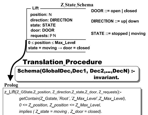
Figure 3: Z State Schema and its Translation Procedure
