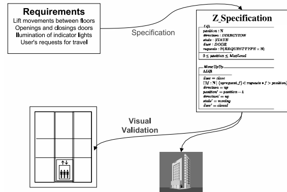
Figure 2: Requirements Validation Process
