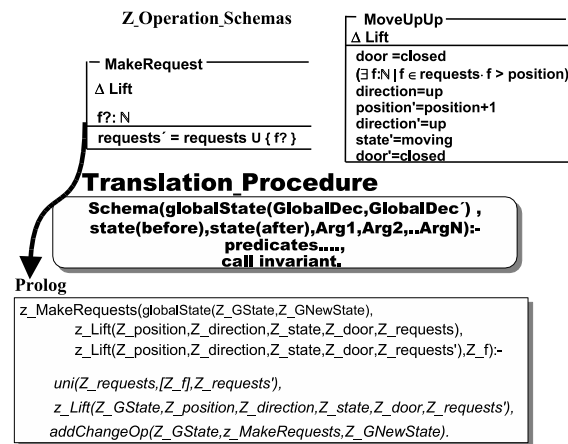
Figure 4: Translation of an Operation Schema
