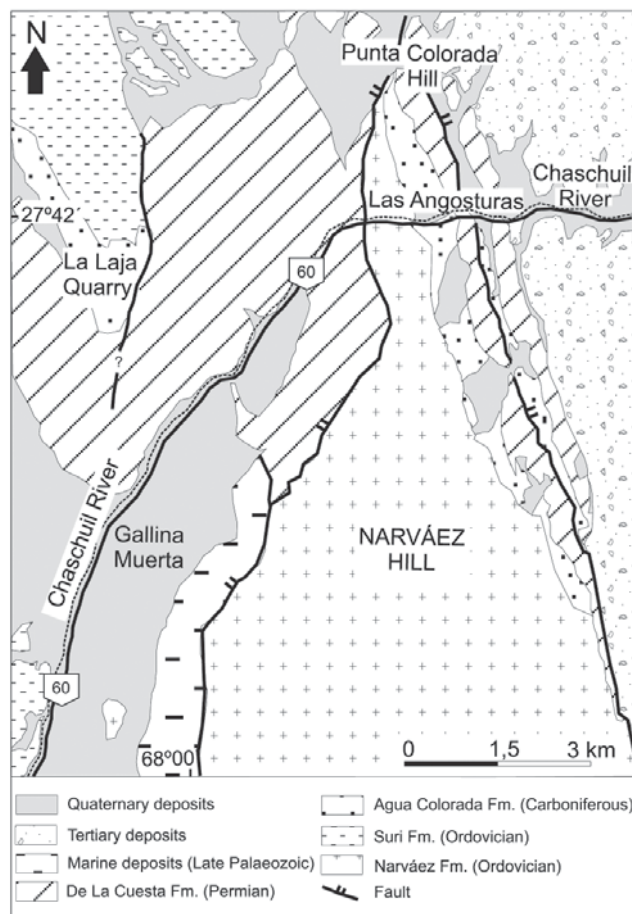
FIGURE 2 | Geological sketch map of the Sierra de Narv ez region. The study area is located to the west and southwest of Las Angosturas.
