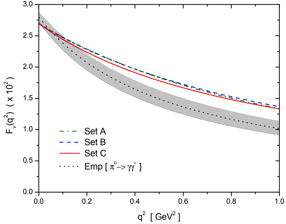
FIG. 2: F_V(q^2) for sets A , B and C . The shadowed region corresponds to empirical data on F^{\pi^0\gamma^*} , using Eqs. (21) and (22)
