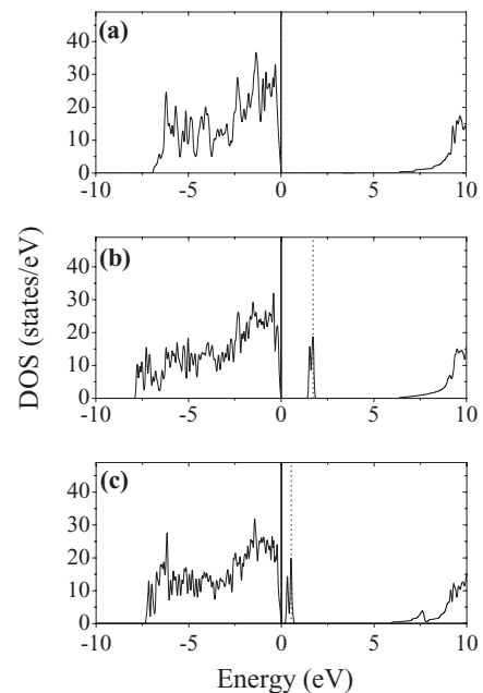
FIG. 2. Total density of states (DOS) of (a) pure \alpha - \text{Al}_2\text{O}_3 , (b) \text{Al}_2\text{O}_3:\text{Cd}_0 , and (c) relaxed \text{Al}_2\text{O}_3:\text{Cd}_0 . The vertical lines are at the top of the valence band (solid) and at the highest occupied state (dotted). In (a) both lines are coincident.
