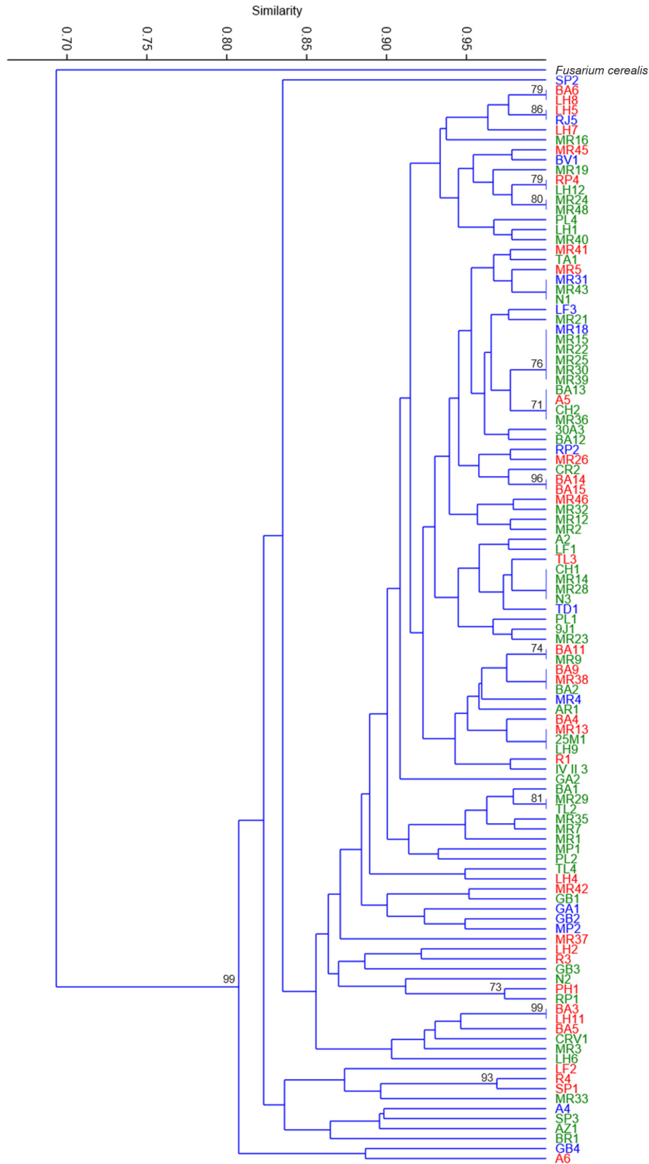
Fig. 1. Dendrogram obtained with the band fingerprints generated by 112 Fusarium graminearum isolates with 4 inter-simple sequence repeats (ISSR) polymorphic primers by means of polymerase chain reaction (PCR). Bootstrap values of 70 or greater are indicated above the branches. Fusarium cerealis strain RBC999 was used as the outgroup. Colors indicate the inclusion of the isolates in one of the groups described: red, green and blue for the high, medium and low aggressiveness, respectively.
