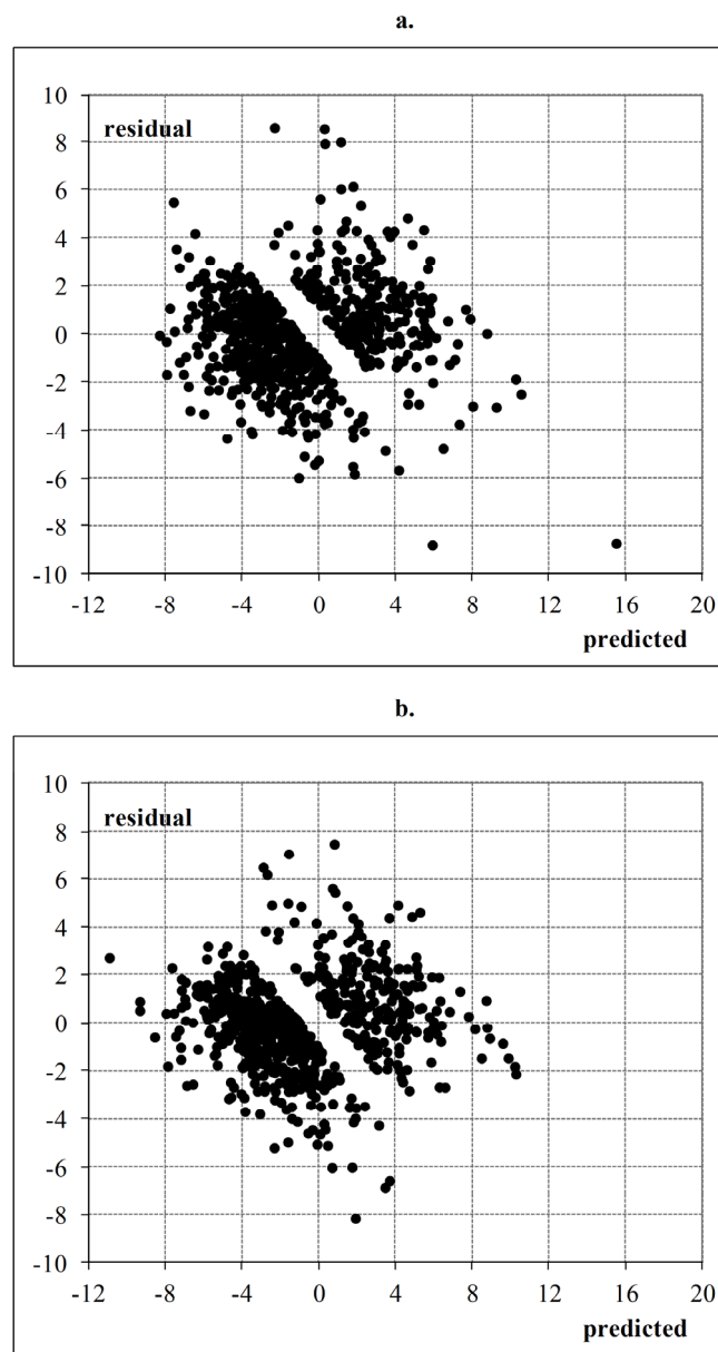
Fig. (2). Dispersion plot of residuals for a. training set; b. test set.
