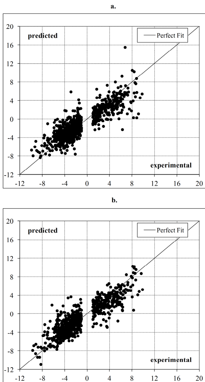
Fig. (1). Predicted and experimental carcinogenicity values for a. training set; b. test set.
