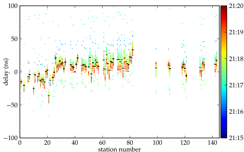
Figure 12. Per-event time offsets for all AERA detector stations determined from AERA and ADS-B data for an airplane detected on September 22. Time offsets are relative to reference station 40. Stations 1–24 are equipped with logarithmic-periodic dipole antennas, stations with numbers 25 and higher are equipped with butterfly antennas. Gaps in the station numbering are related to stations not participating in the airplane trigger (marked gray in figure 1). The color code denotes the local time at which the airplane event was detected.
