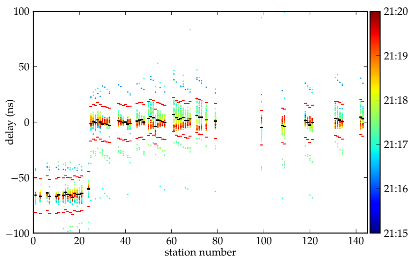
Figure 13. Same as figure 12 when applying the airplane timing calibration after per-event clock-drift correction using the beacon method. The red lines show the range of mean \pm 4 \cdot \text{MAD} (median absolute deviation).
