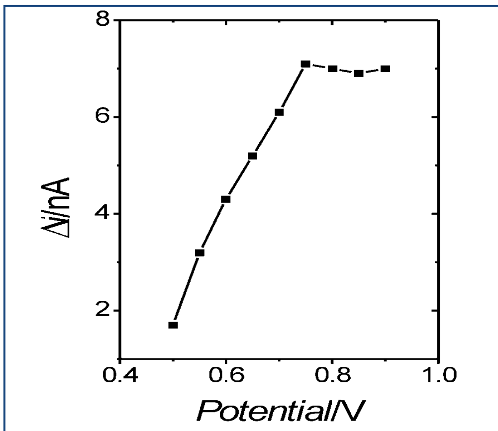
Figure 4. Effect of applied potential on the response current of the Au/POAP/CNT/GOD electrode. Steady-state currents are measured in 1/15 M phosphate buffer solution ( pH 7) containing 2 mM glucose [30].
