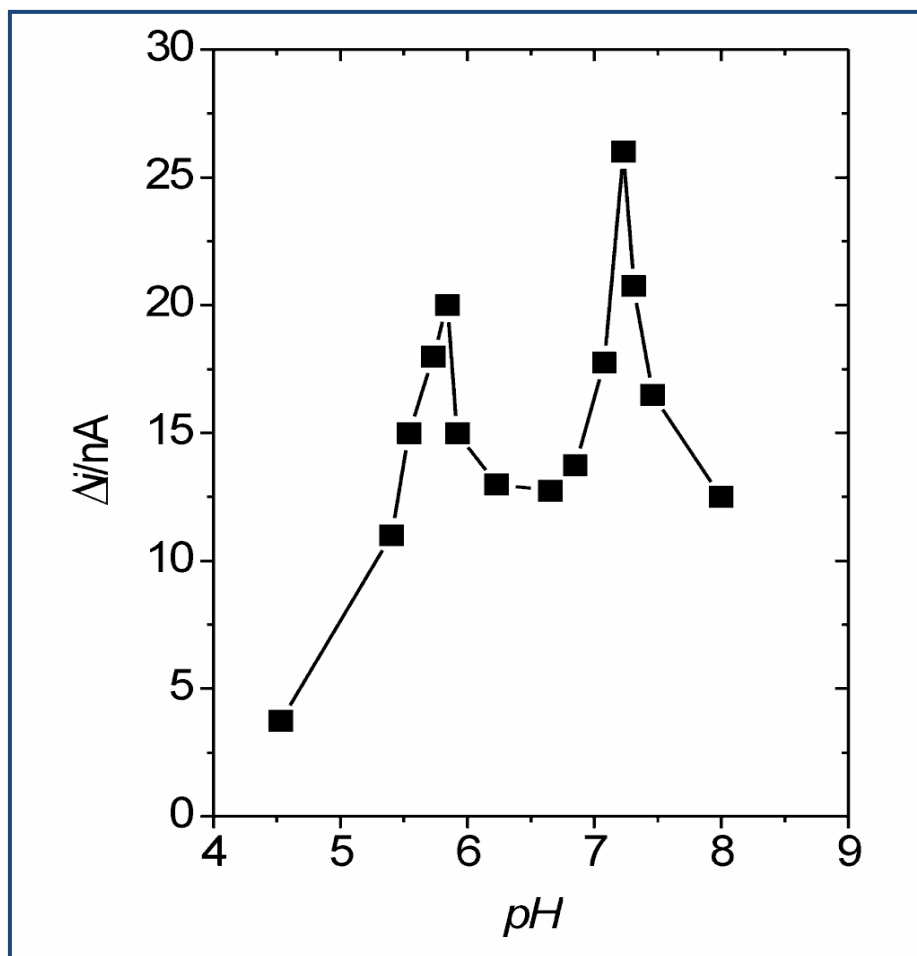
Figure 3. Effect of pH on the steady-state response current on the Pt/Prussian blue/poly( o -aminophenol)/glucose oxidase electrode at 0.6 V in 1/15 M phosphate buffer solution ( pH 7) containing 2 mM glucose ( n = 3) [28].
