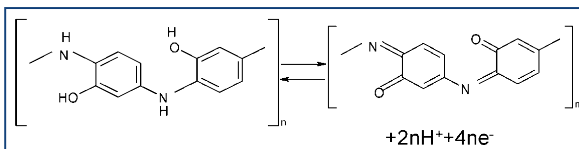
Figure. 1. Stoichiometry of redox reactions of POAP film electrodes [8].
