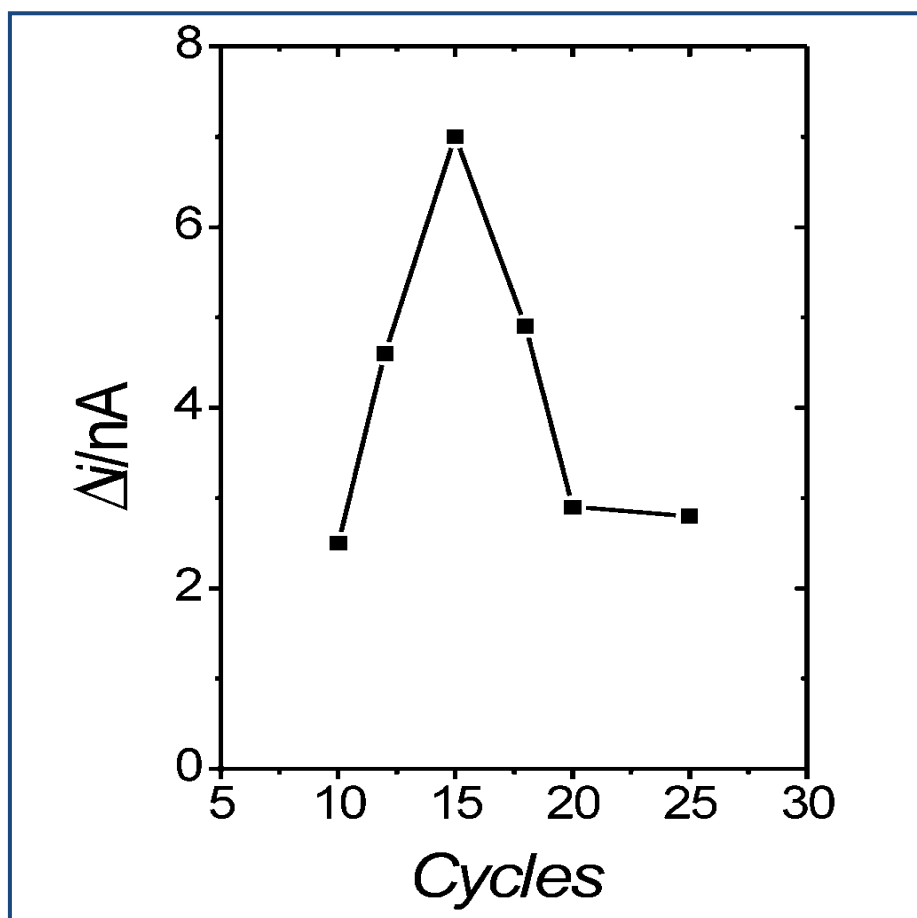
Figure 2. Effect of the polymerization cycle number on the response current of the Au/POAP/CNT/GOD electrode. Steady-state currents are measured at 0.75 V (SCE) in 1/15 M phosphate buffer solution (pH 7) containing 2 mM glucose ( n=3 ) [30]
