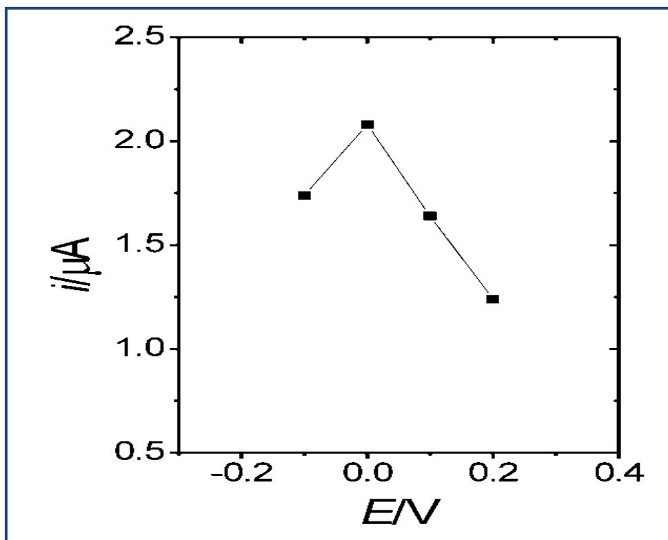
Figure 6. Effect of operating potential on the response of the HRP-ferrocene/POAP electrode (5 mM, 10 cycles, 50 \text{mV s}^{-1} to 10^{-4} M injections of \text{H}_2\text{O}_2 [34].
