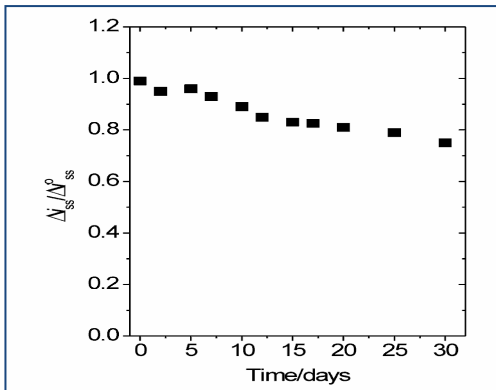
Figure 5. Stability of the Pt/Prussian blue/poly(o-aminophenol)/glucose oxidase electrode stored in 1/15 M phosphate buffer solution (pH 7) at 4 °C. Stability determined by 5mM glucose in 1/15 M phosphate buffer solution (pH 7). Applied potential, 0.6 V (SCE) [28].
