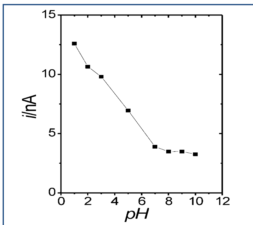
Figure 7. Amperometric currents developed by a POAP-modified electrode for 1.0 \times 10^{-5} M NADH as a function of the electropolymerization pH medium. Applied potential 0.15 V (Ag/AgCl). Supporting electrolyte for the amperometric measurements: 0.1 M phosphate buffer pH 7 [37].
