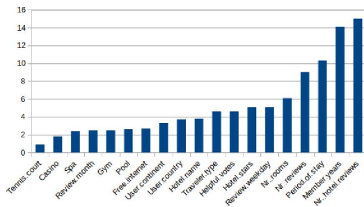
Fig. 1. Features selected in [8]
