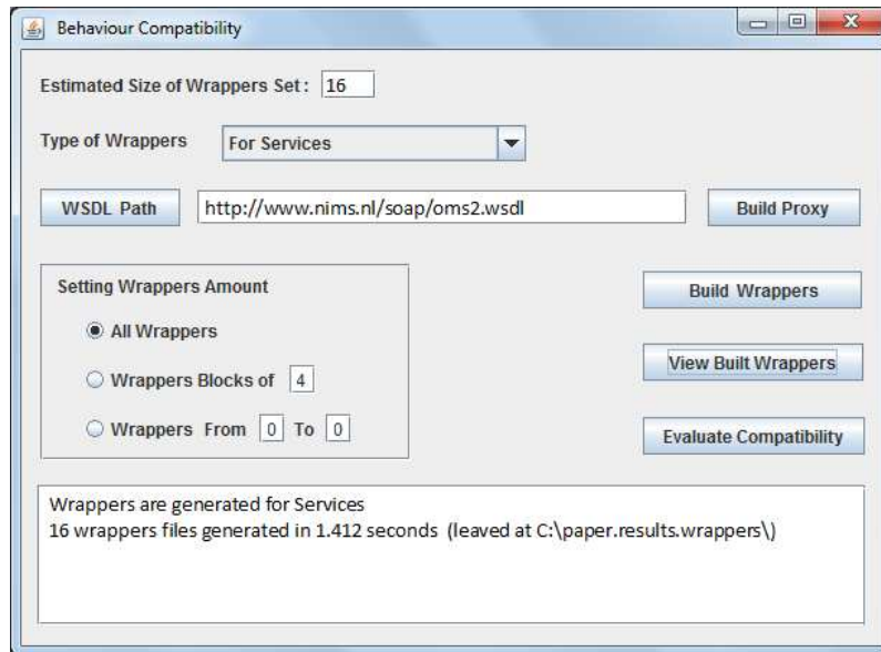
Fig. 5. Wrappers generation for Behavior Compatibility
