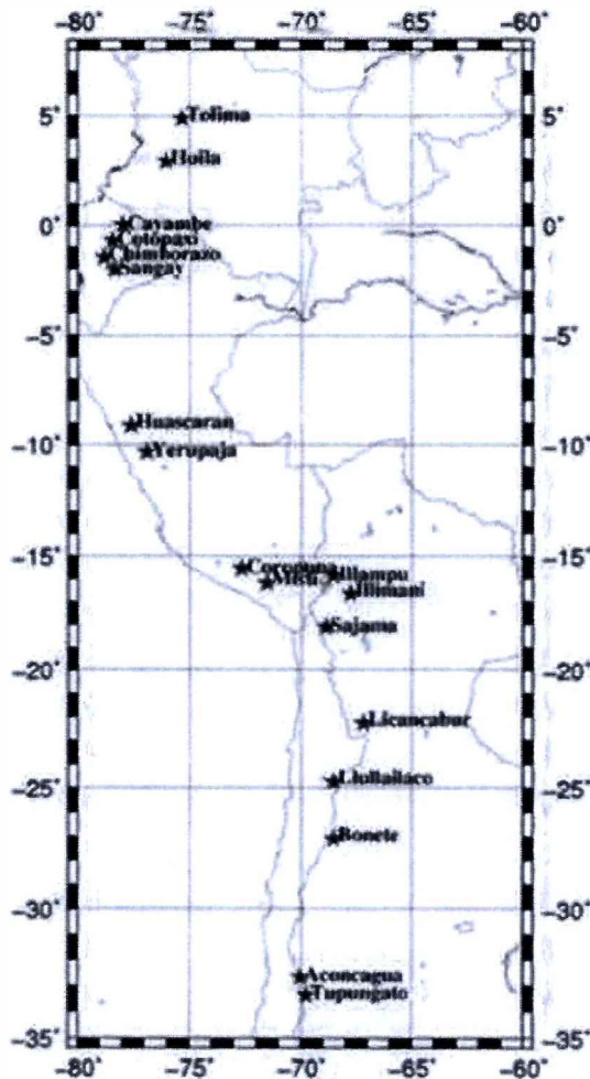
Figure 8. Andean peaks
