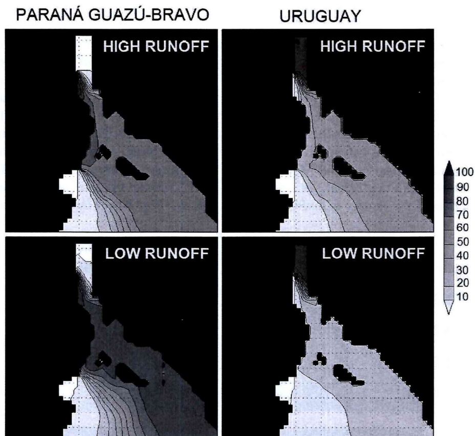
Figure 8. Detail of the surface concentration contours (%) at the upper estuary of the dye tracers characterizing the Uruguay (right panels) and Paraná Guazú-Bravo (left panels) as derived from simulations forced by mean summer atmospheric forcing and high (upper panels) and low (lower panels) runoff for the ebb tide.
