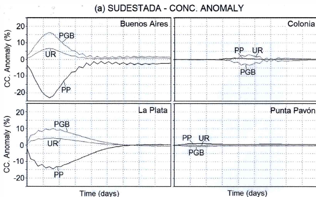
Figure 12a. Surface concentration anomalies (%) of the dye tracers characterizing the Uruguay (UR), Paraná Guazú-Bravo (PGB) and Paraná las Palmas (PP) rivers introduced by the Sudestada at several coastal locations of the Río de la Plata estuary.
