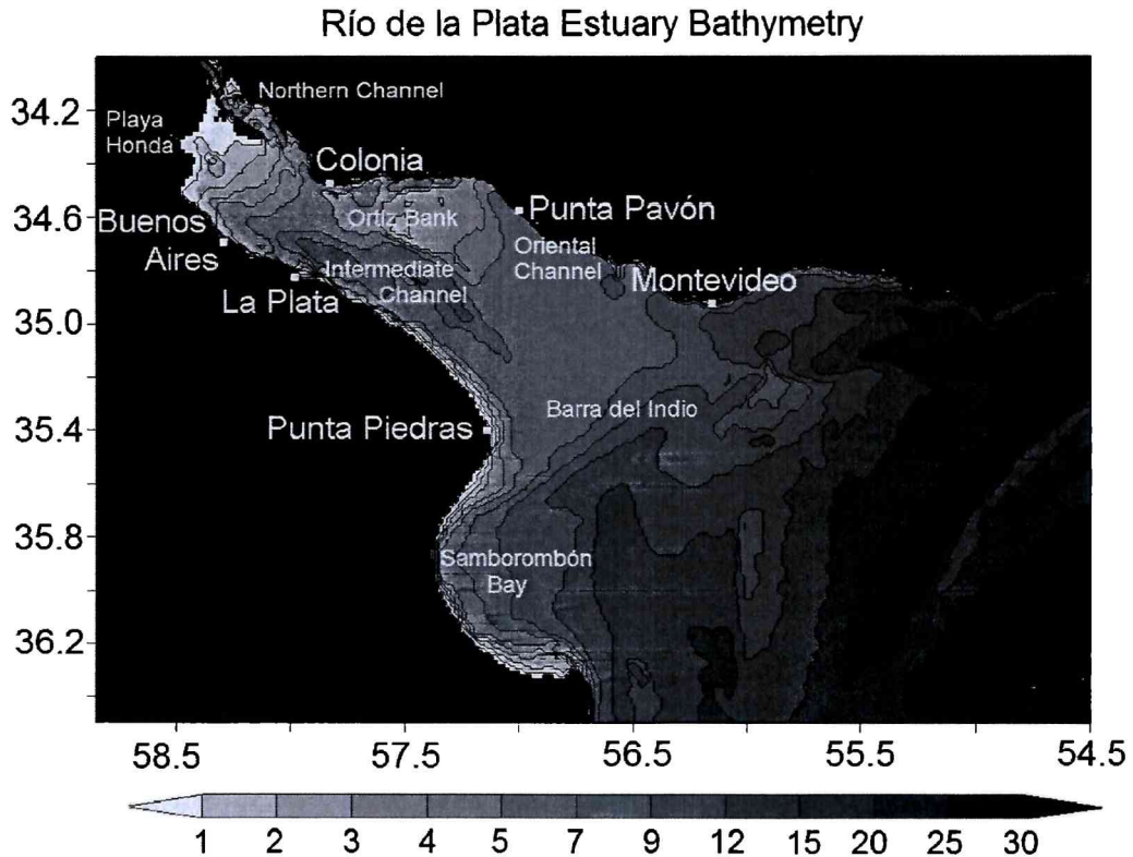
Figure 2. Model domain and Río de la Plata bathymetry (in m) in a 1.5 km × 1.5 km resolution, as seen by the model, together with the main geographic and topographical features.
