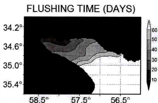
Figure 13. Flushing time contours every 10 days of the upper and intermediate Río de la Plata estuary for mean runoff conditions.
