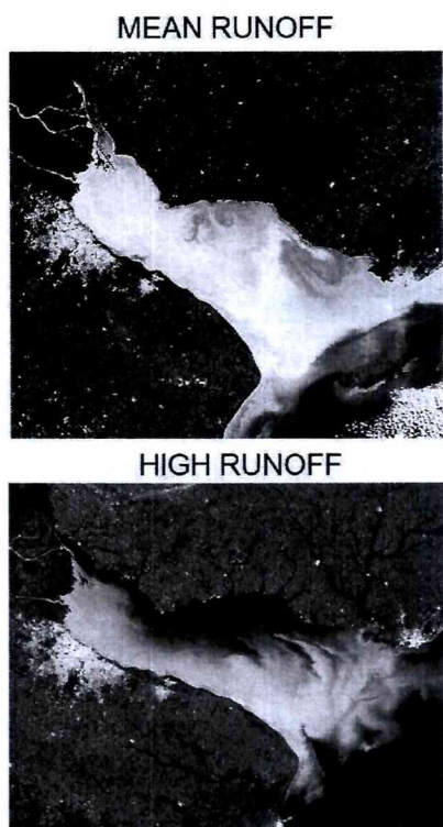
Figure 16. Gray scale color images collected by the Moderate Resolution Imaging Spectroradiometer on board of Terra satellite (MODIS-TERRA) in April 13 th , 2003 (upper panel) and May 4 th , 2002 (lower panel). Figure shows typical images collected by the satellite for mean runoff and high Uruguay River runoff conditions, respectively. (From Visible Earth, http://visibleearth.nasa.gov ).
