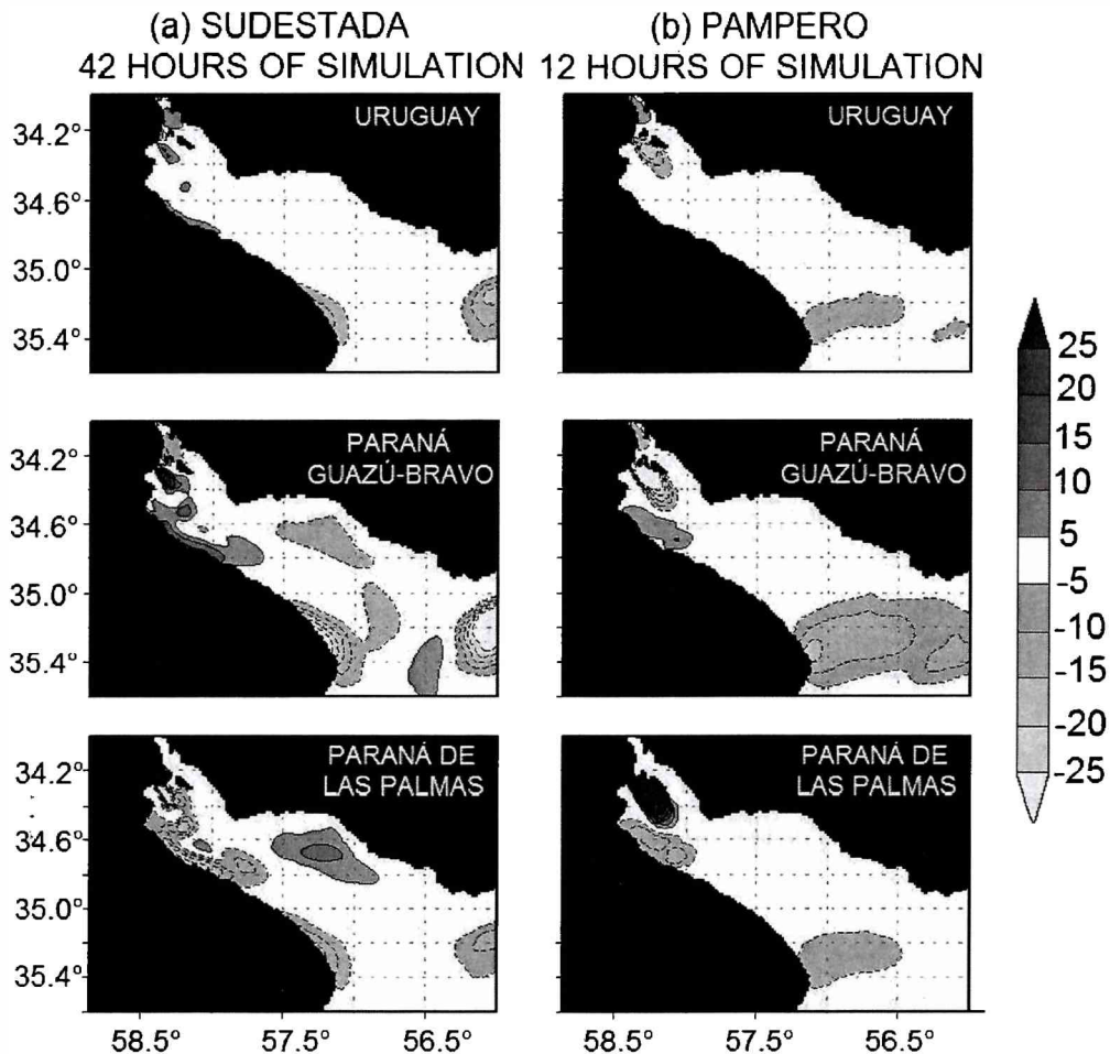
Figure 11. Surface concentration anomaly contours (%) of the dye tracers characterizing the Uruguay (upper panels), Paraná Guazú-Bravo (central panels) and Paraná de las Palmas (lower panels) rivers introduced by the Sudestada (a) and Pampero (b).
