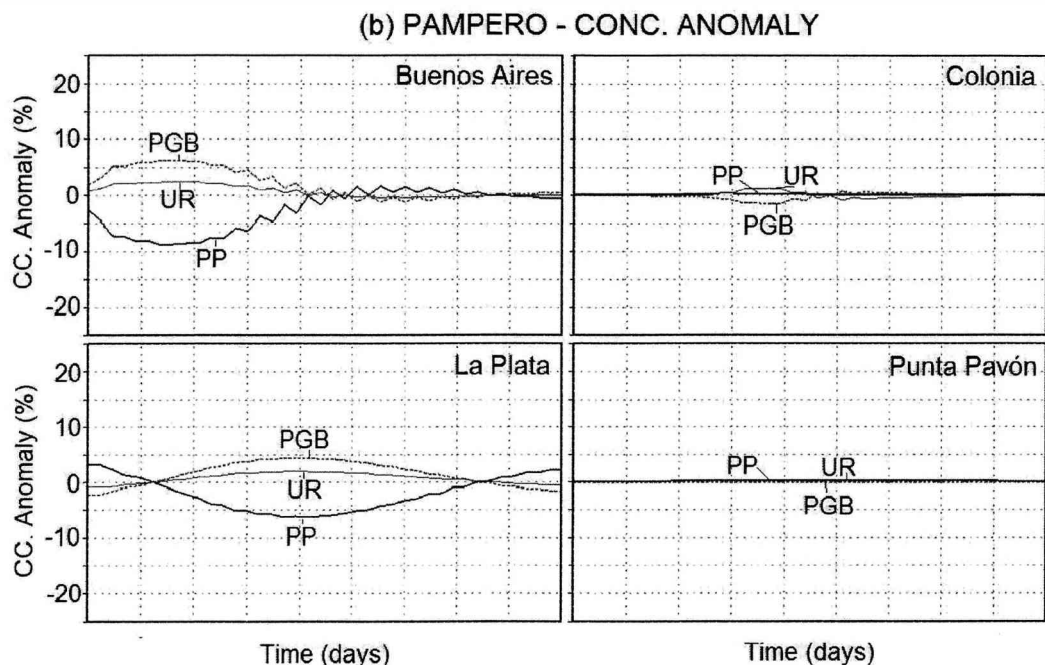
Figure 12b. Idem Figure 12a but for the Pampero.
