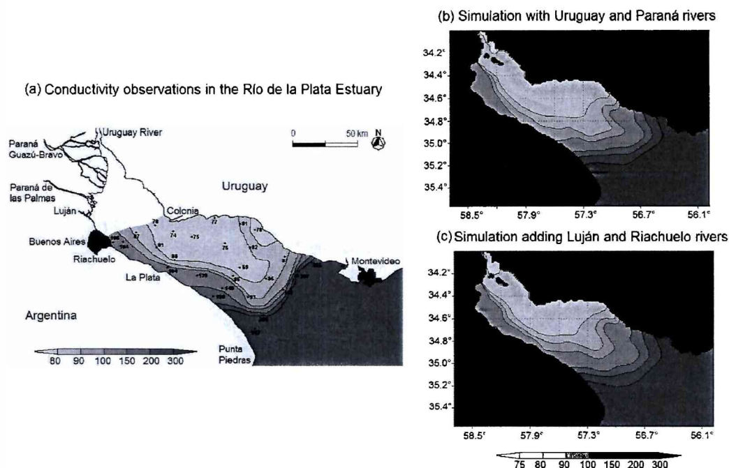
Figure 3. Surface specific conductivity contours ( \mu\text{S cm}^{-1} ) from direct observations collected between November 22 nd and 23 rd , 1982 (a); the dots show the sites where data were gathered. Specific conductivity contours ( \mu\text{S cm}^{-1} ) as derived from numerical simulations including the conductivity sources at the three main tributaries of the Río de la Plata (b) and adding the Luján and Riachuelo rivers (c).
