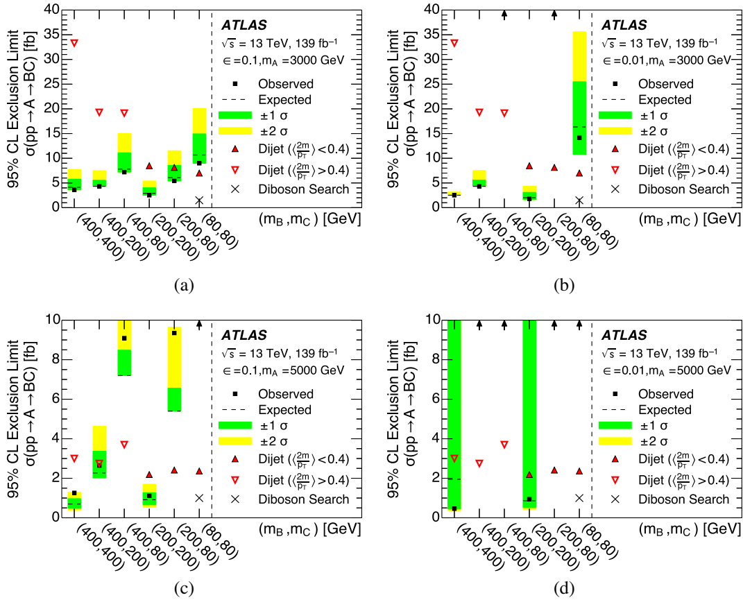
FIG. 3. 95% confidence level upper limits on the cross section for a variety of signal models, labeled by (m_B, m_C) , in GeV. The limits are shown for signal models with (a), (b) m_A = 3000 GeV and NN trained on signal region 2; and (c), (d) m_A = 5000 GeV and NN trained on signal region 5. The limits are broken down between the analyses with (a), (c) \epsilon = 0.1 and (b), (d) \epsilon = 0.01 . Also shown are the limits from the ATLAS dijet search [100] and the ATLAS all-hadronic diboson search [103]. The inclusive dijet limits are calculated using the W' signals from this paper and the full analysis pipeline of Ref. [100]; the diboson search limits are computed using the heavy vector triplet [104] W' signal from Ref. [103]. The acceptance for the W' in this Letter, compared to the W' acceptance in Ref. [103], is 86% and 54% for m_{W'} = 3 and 5 TeV, respectively. Missing observed markers are higher than the plotted range. Poor limits occur when the NN fails to tag the signal.
