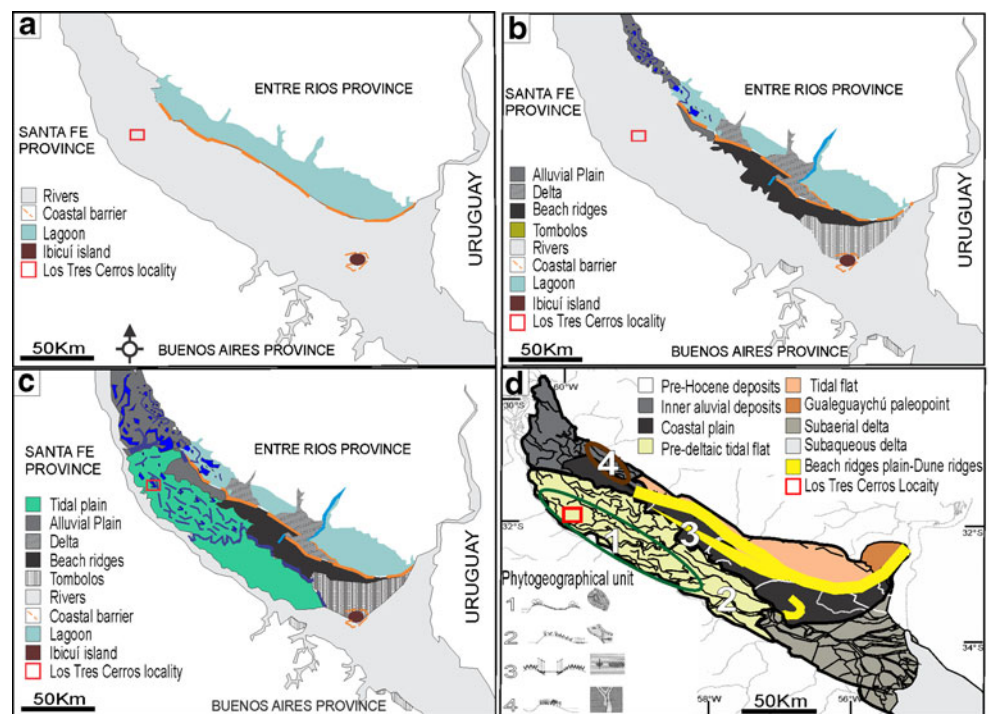
Fig. 3 a–c Evolution of the deltaic area during the Holocene proposed by Codignotto (2004). a 7.5 kcal. years BP; b 6 kcal. years BP; c 4 kcal. years BP; d actual geomorphologic map ( sensu Cavallotto et al. (2005), with the detail of the phytogeographical units proposed Malvárez (1999:37): (1) forests and prairies associated with Paraná meandering channels and islands; (2) prairies associated with previous tidal plain; (3) prairies associated with ridges and depressions; and (4) patches of prairies associated with low overbank ridges.
