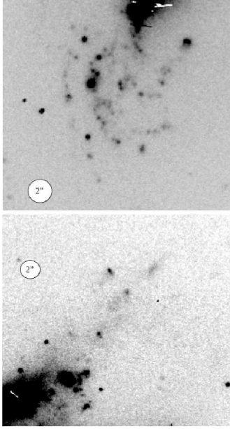
Figure 2: Gemini H\alpha image cutouts of the Taffy system. Top panel: the outskirts southern side of UGC 12914 (#1 RA=00:01:40, DEC=+23:28:24.4, J2000). Bottom panel: the outskirts northern side of UGC 12915 #2 RA=00:01:39.16, DEC=+23:30:16.4, J2000).
