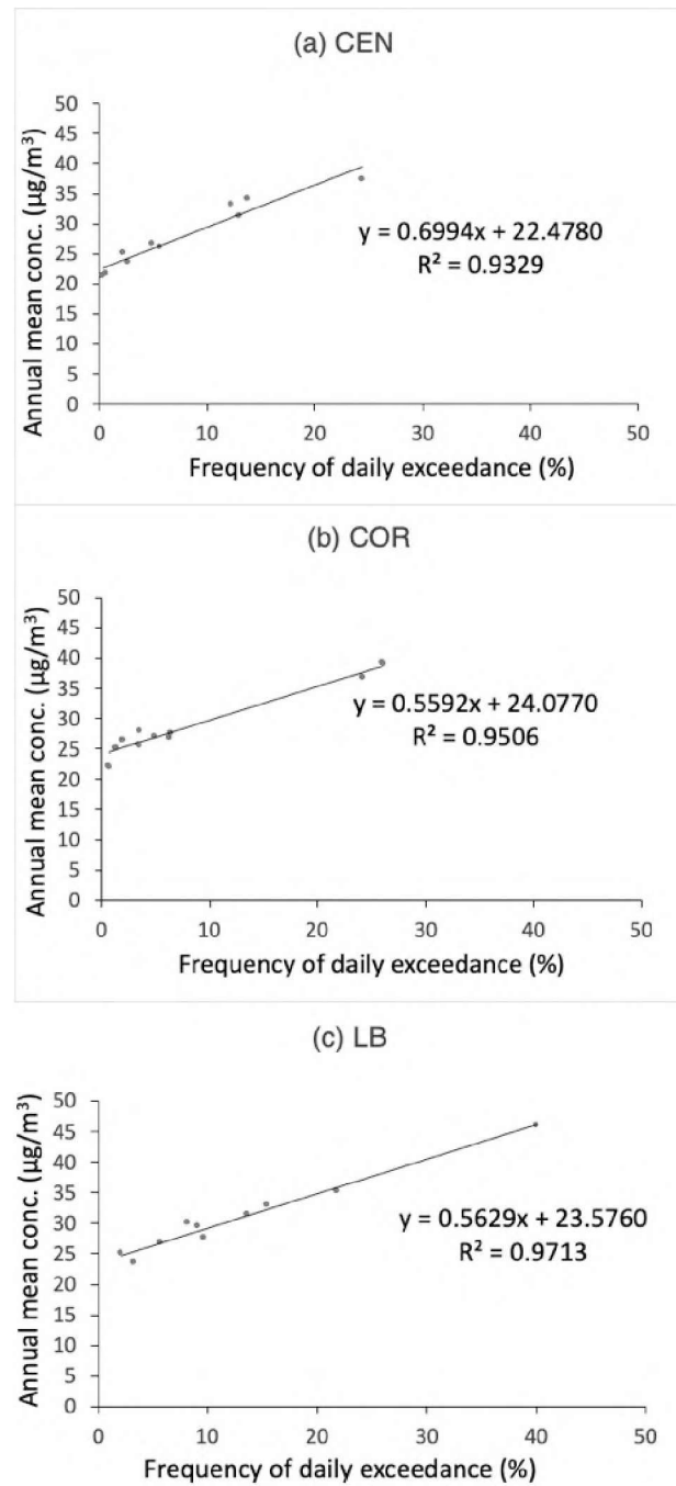
Figure A.2: Scatter plot of annual mean PM 10 concentration vs frequency of daily mean PM 10 concentration exceeding the WHO guideline level (45 µg m 3 ) at: a) CEN, b) COR and c) LB. The linear fit is included.
