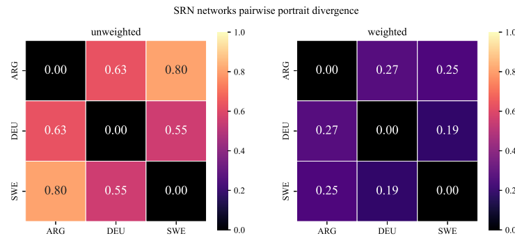
Fig. 6. SRNs network pairwise portrait divergence. Left: unweighted portraits divergence. Color range for D_{JS}(G, G') \in [0, 1] , greater values showing more dissimilar network portraits.
