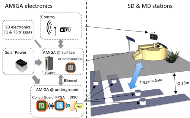
Fig. 53. AMIGA station: SD+MD paired detectors. During the MD prototype phase the 30 m 2 buried scintillators are segmented into 4 modules, 2 × 10 m 2 +2 × 5 m 2 . To avoid shadowing effects by the water Cherenkov detector, there are 5 m of sideways clearance. The buried front end electronics is serviceable by means of an access pipe which is filled with local soil bags. Data are sent by a dedicated WiFi antenna.
