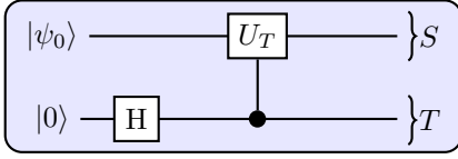
FIG. 1. (Color online) Schematic circuit representing the generation of the system-time pure state (1). The control gate performs the operation U_t on S if T is in state |t\rangle , while the Hadamard-type gate H creates the superposition \propto \sum_{t=0}^{N-1} |t\rangle .
