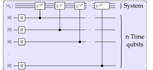
FIG. 2. (Color online) Circuit representing the generation of the system-time state (1) for U_t = (U)^t and N = 2^n . The n control gates perform the operation U^t = U^{\sum_{j=1}^n t_j 2^{j-1}} on the system after writing t in the binary form t = \sum_{j=1}^n t_j 2^{j-1} , while the n Hadamard gates lead to a coherent sum over all values of the t_j 's, i.e., over all t from 0 to 2^n - 1 .
