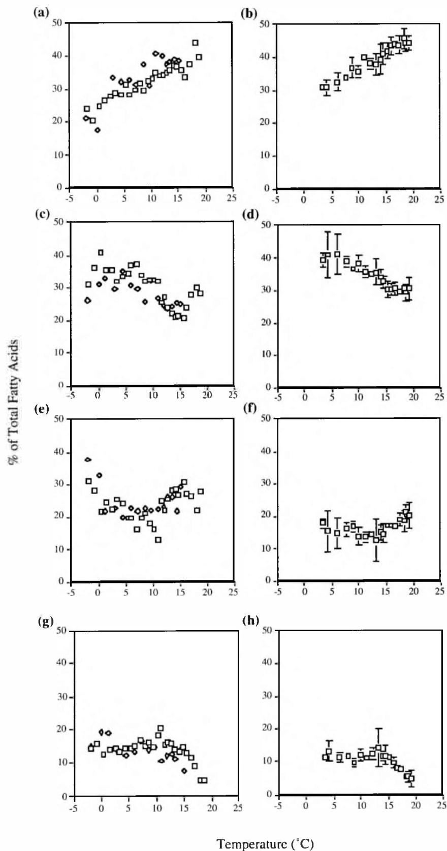
FIG. 3. Plots of S. gelidimarina fatty acid compositions for the entire biokinetic temperature range at an a_w of 0.993 (1.0% [wt/vol] NaCl) for two data sets (□ and ◇) and at an a_w of 0.977 (4.0% [wt/vol] NaCl). The data points for a_w 0.977 represent means based on values in three data sets, and standard deviations are indicated by error bars. (a and b) Total saturated fatty acids at an a_w of 0.993 (a) or 0.977 (b). (c and d) Total monounsaturated fatty acids at an a_w of 0.993 (c) or 0.977 (d). (e and f) Total branched-chain fatty acids at an a_w of 0.993 (e) or 0.977 (f) (g and h). Total polyunsaturated fatty acids at an a_w of 0.993 (g) or 0.977 (h).
