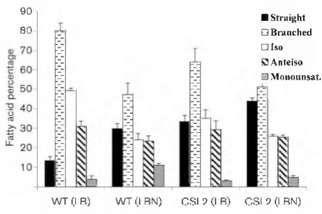
Fig. 3. Fatty acid composition of the B. subtilis wild-type YB886 and CSL2 mutant strains grown to stationary phase in LB and LBN. The fatty acids were analysed as indicated in Methods. The values represent the mean \pm SD of three independent experiments. Straight, straight-chain saturated fatty acids; Branched, branched-chain saturated fatty acids; Iso, branched-chain saturated fatty acids iso series; Anteiso, branched-chain saturated fatty acids anteiso series; Monounsaturat, monounsaturated fatty acids. The fatty acid composition of the wild-type versus the mutant strain in each medium was compared using the Student t -test.
