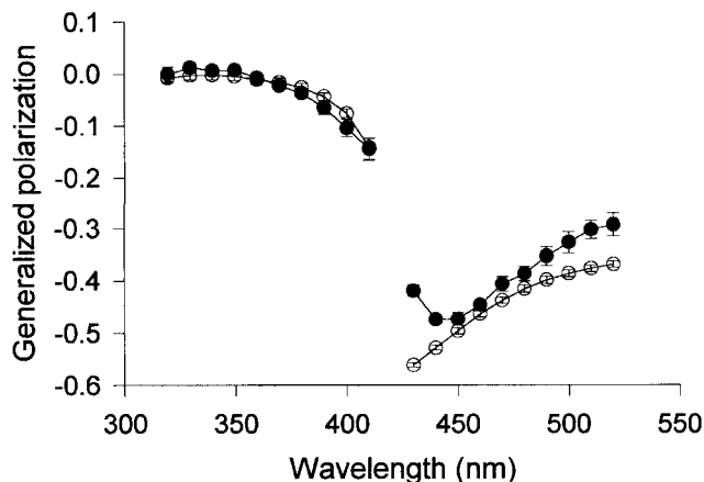
Fig. 4. Excitation and emission generalized polarization of Laurdan in pure POPC multilamellar vesicles at 20°C in the presence (solid symbols) and absence (open symbols) of FS 5 ppm. The excitation GP spectra were measured using emission wavelength of 440 and 490 nm, and the emission GP spectra were measured using excitation wavelengths of 340 and 410 nm.
