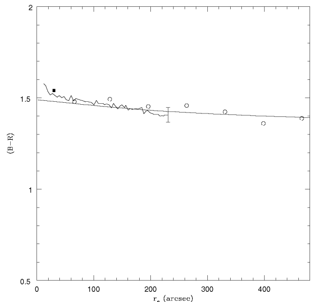
Figure 10. Galaxy (B - R_{\text{KC}}) colour as a function of elliptical galactocentric radius r_e (solid curve). The straight line is the expected gradient from the model described in Section 2. The square indicates the (B - R_{\text{KC}}) colour measured by Michard (2000) at r_0 = 22.8 arcsec. The bar at 228.8 arcsec indicates the uncertainty of our colour gradient. Open circles show the resulting colour gradient obtained by combining our photometry and that given in D2003 (see text).
