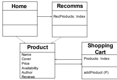
Fig. 6. Navigational Schema for the e-store site
