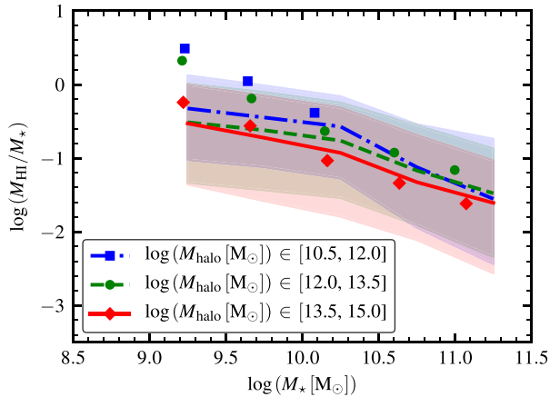
Figure 16. Atomic hydrogen gas fraction as a function of stellar mass for satellite galaxies in model SAG_{\beta 1.3} within different ranges of main host halo mass, as indicated in the legend. Different lines and associated shaded areas represent the corresponding median values and 10 and 90 percentiles, respectively. Median values are compared with the average atomic gas fraction presented by Brown et al. (2017), who consider H I data from ALFALFA survey (different symbols). The match between model results and observations is rather good for satellites with stellar mass larger than 10^{10} M_{\odot} residing in haloes more massive than \approx 10^{12} M_{\odot} , consistent with the good behaviour of the radial dependence of the fraction of quenched massive satellites.
