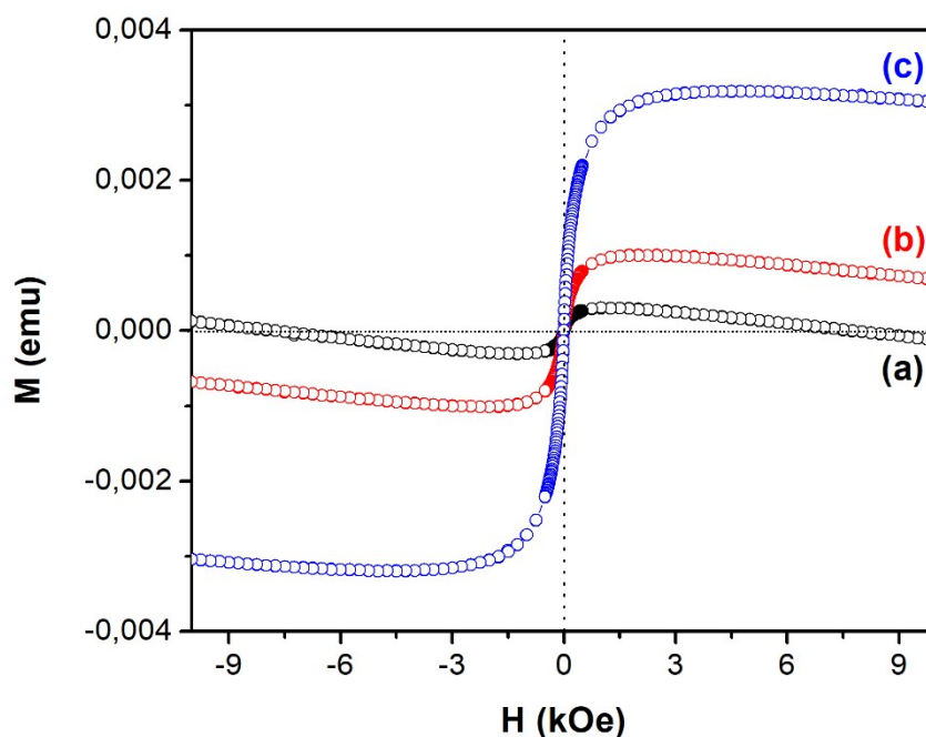
Figure 7. Magnetic hysteresis loops corresponding to the samples containing concentrations in the order of 0.476 (a), 0.909 (b) and 1.304 (c) w/v % in both directions, plane and perpendicular.
