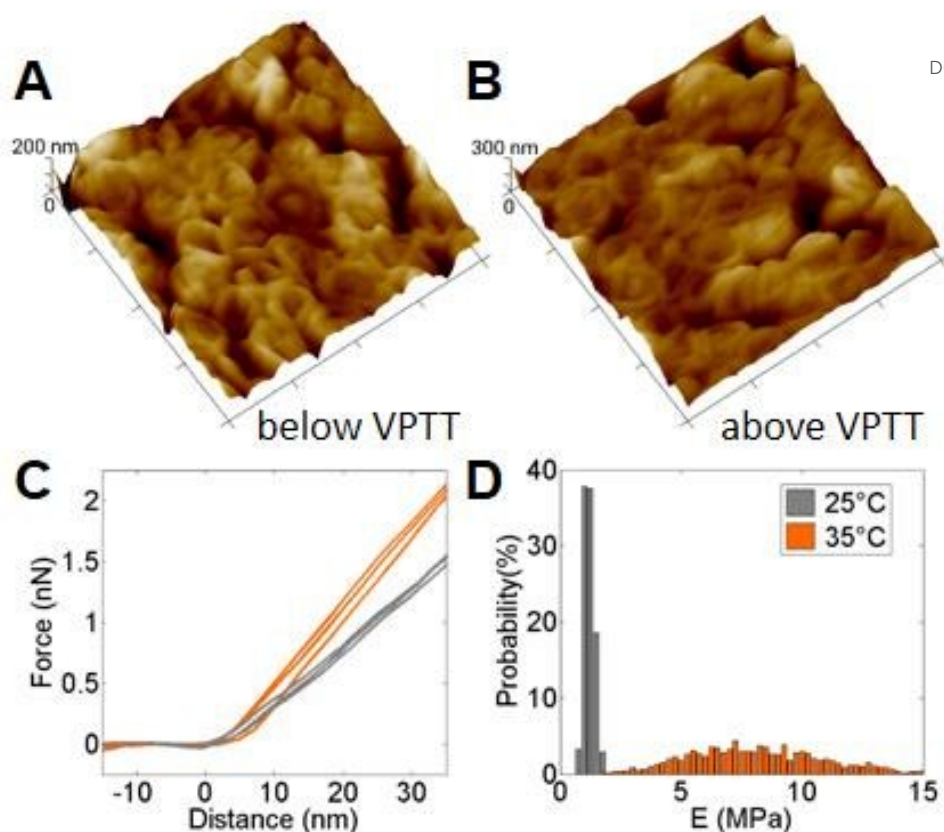
Figure 4. In-situ AFM three-dimensional topographic images of Fe 3 O 4 -PNIPAm nanopillars surfaces (A) below and (B) above VPTT, (C) representative force-distance curves and (D) frequency histograms of the Young Modulus at 25°C (gray, Mean stiffness = 1.20 MPa, Std = 0.21 MPa, N = 714 force curves from 8 nanopillars) and 35°C (orange, Mean stiffness = 8.6 MPa, Std = 4.3 MPa, N = 1424 force curves from 8 nanopillars). All images were acquired in solution on PF-QNM mode; scan size: 2 μm × 2 μm, z-scale indicated on each image.
