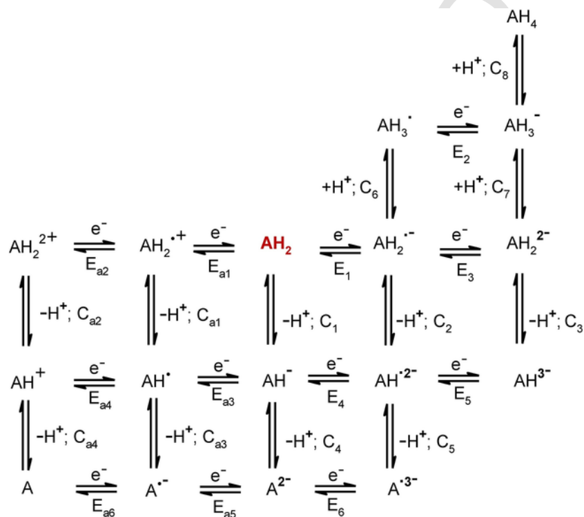
Scheme 2. General electrochemical scheme proposed for ALZ ( AH_2 ) in non-aqueous solvent in the absence and the presence of proton donor and bases.
